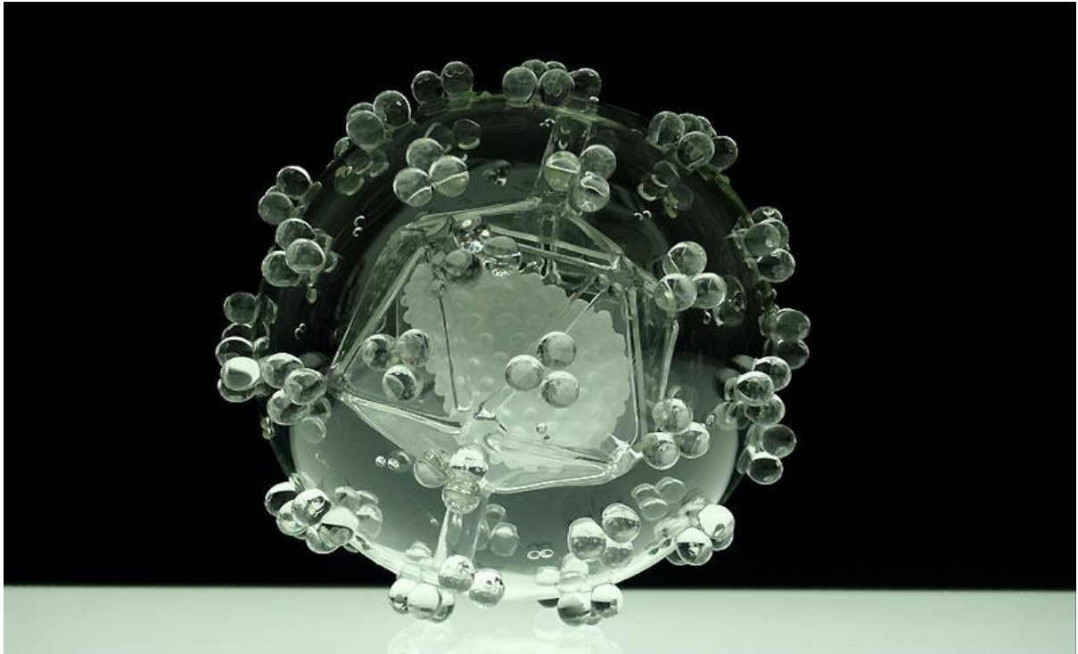
HIV 21cm diameter (large)
